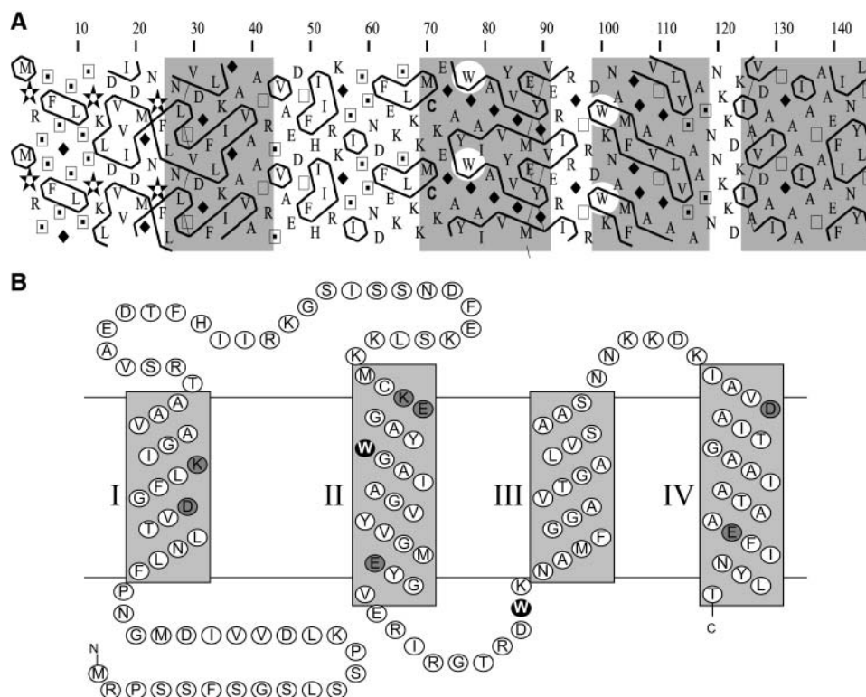
FIGURE 5 (A) Hydrophobic cluster analysis. The \alpha -helices of OEP16 are highlighted in gray. The two tryptophan residues in helices II and III are marked ( \circ ). W77 is embedded in a more hydrophobic environment than W100. (B) Topology model for OEP16. The tryptophan residues are highlighted, as are charged residues within the predicted transmembrane helices. Note that only helix I contains charged residues in a central position and that the exchangeable (Steinkamp et al., 2000) helices II and IV have similar patterns of charged residues at their ends.
